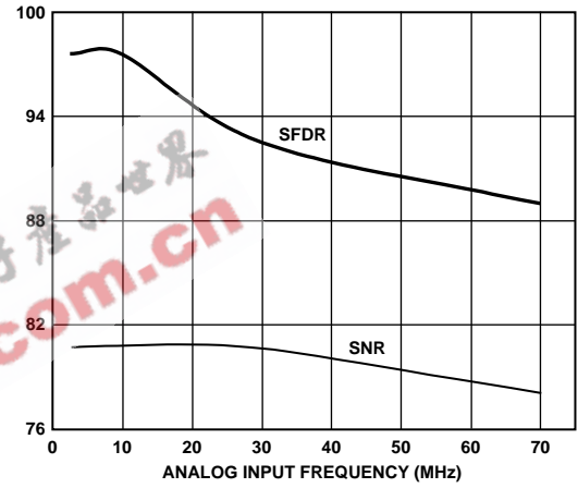
Figure 17. SFDR and SNR vs. Analog Input Frequency
