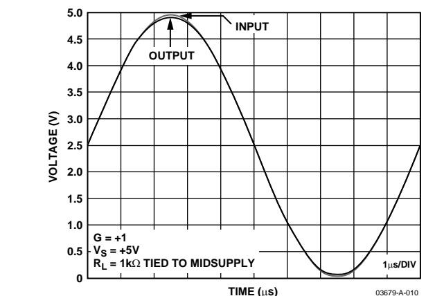
Figure 5. Rail-to-Rail Response
