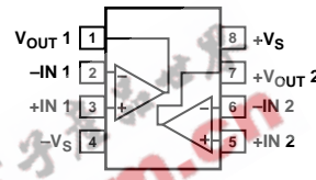
Figure 3. SOIC-8 (R) and SOT23-8 (RJ)
