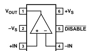
Figure 2. SC70-6 (KS)
