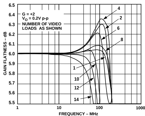
Figure 8. Gain Flatness vs. Frequency vs. Number of Video Loads
