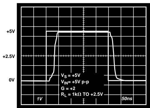
Figure 33. Overdrive Recovery
