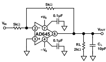
Figure 29a. Unity-Gain Inverter
