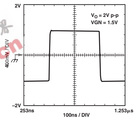
TPC 24. Large Signal Pulse Response
