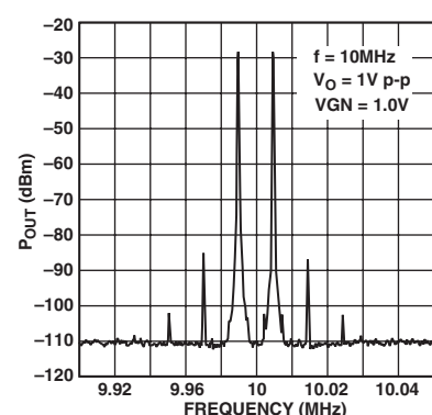
TPC 21. Intermodulation Distortion
