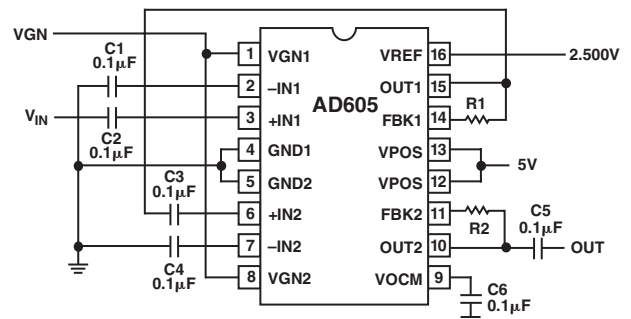
Figure 5. Doubling the Gain Range with Two Amplifiers
