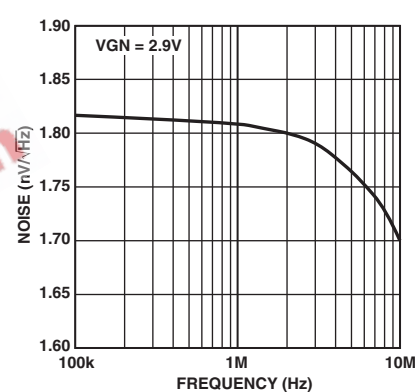
TPC 15. Input Referred Noise vs. Frequency
