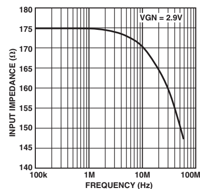
TPC 30. Input Impedance vs. Frequency
