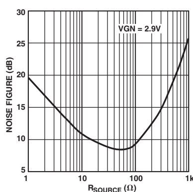
TPC 17. Noise TPC vs. R_{SOURCE}
