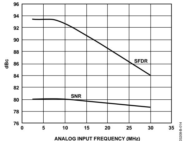
Figure 14. SFDR and SNR vs. Analog Input Frequency
