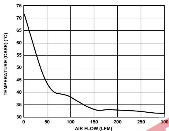
Figure 15. Temperature (Case) vs. Air Flow (Ambient)
