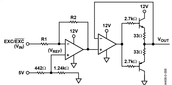
Figure 6. Buffer Circuit
