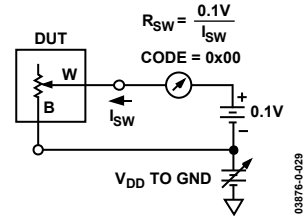
Figure 23. Test Circuit for Incremental ON Resistance
