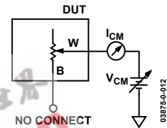
Figure 24. Test Circuit for Common-Mode Leakage Current
