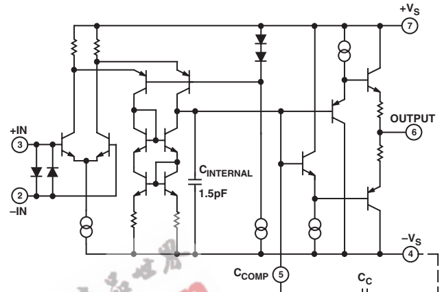
Figure 6. Simplified Schematic
