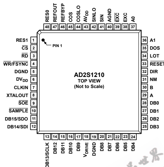
Figure 2. Pin Configuration
