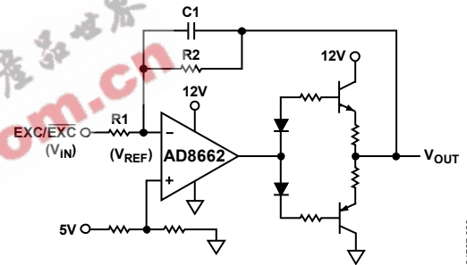
Figure 27. Buffer Circuit
