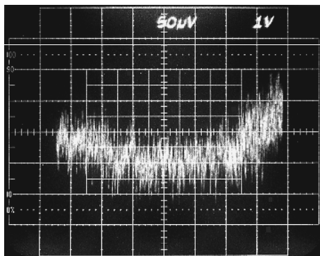
Figure 38. Gain Nonlinearity ( G = -100 , 15 ppm/Div)
