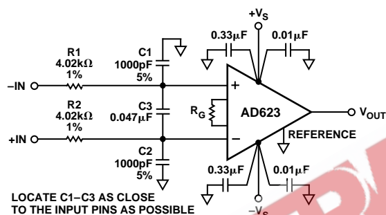
Figure 43. Circuit to Attenuate RF Interference
