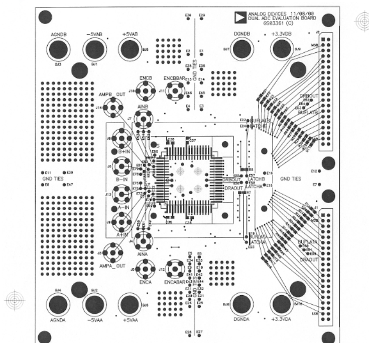
Figure 9. Evaluation Board Mechanical Layout
