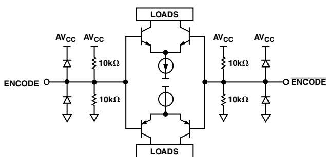
Figure 3. ENCODE Inputs
