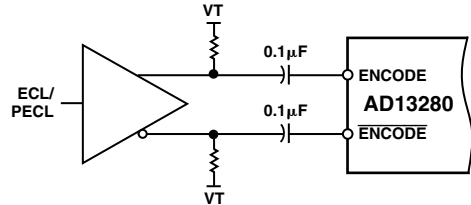
Figure 7. Differential ECL for Encode
