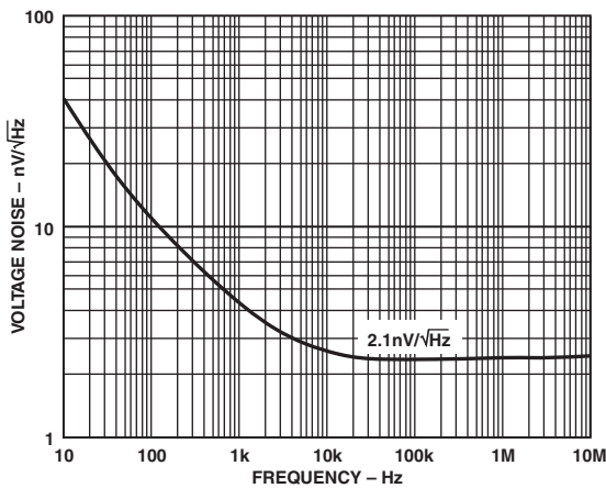
TPC 33. Input Voltage Noise vs. Frequency
