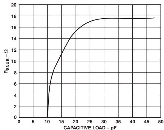
Figure 16. Relationship of R_{SNUB} vs. C_L for 2 dB Peaking at a Gain of +2
