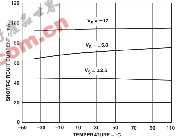
TPC 23. Short-Circuit Current to Ground vs. Temperature
