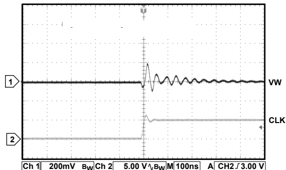
Figure 24. Digital Feedthrough
