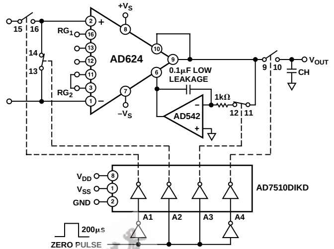
Figure 42. Autozero Circuit
