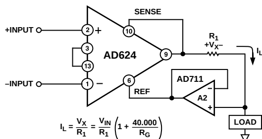
Figure 37. Voltage-to-Current Converter
