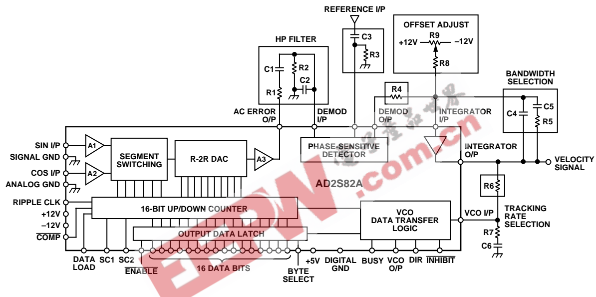
Figure 1a. AD2S82A Connection Diagram
