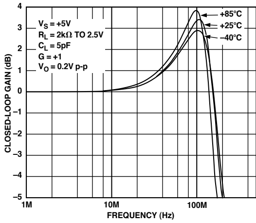
Figure 16. Closed-Loop Frequency Response vs. Temperature
