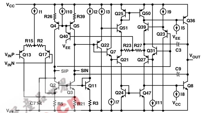
Figure 34. AD8044 Simplified Schematic
