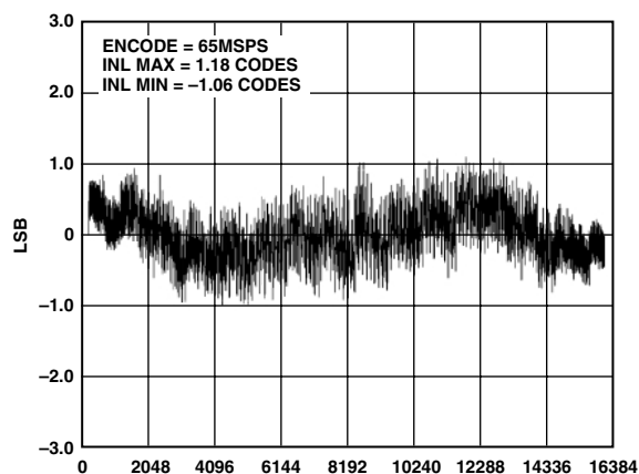
TPC 10. Integral Nonlinearity
