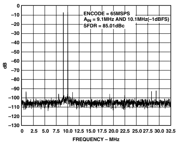
TPC 3. Two-Tone @ 9.1 MHz/10.1 MHz
