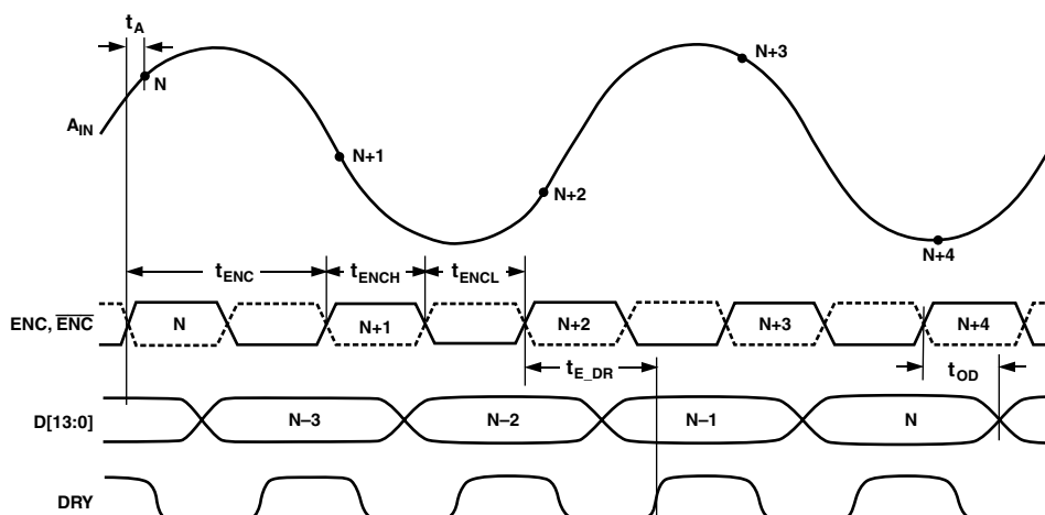
Figure 1. Timing Diagram
