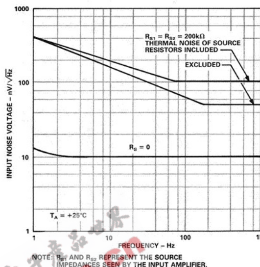
Figure 12. Typical Input Voltage Noise (nV/√Hz) vs. Frequency for the AD208's Uncommitted Input Op Amp
