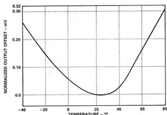
Figure 10. Normalized Output Offset Voltage (mV) vs. Temperature (°C) with an AD208 Gain of 1 V/V, with V_S = 15 V pk-pk, 25 kHz Square Wave
