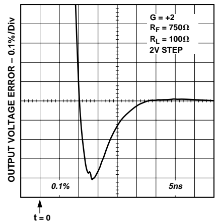
Figure 33. Settling Time, V_S = \pm 5V
