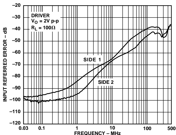
Figure 36. Crosstalk vs. Frequency
