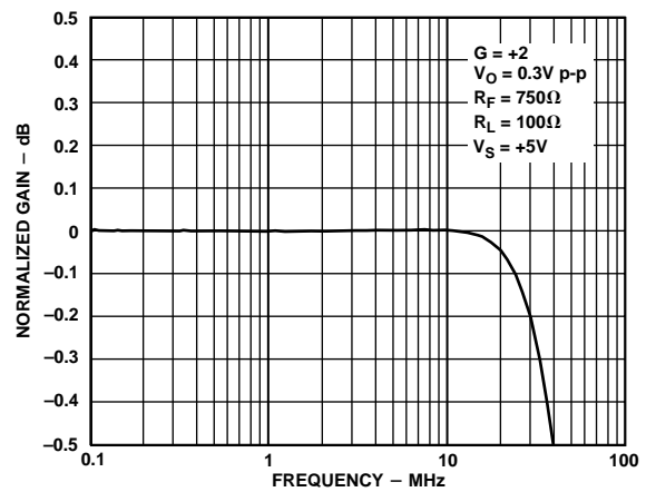
Figure 21. Gain Flatness; V_S = +5\text{ V}
