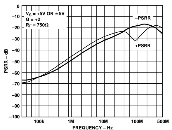
Figure 27. PSRR vs. Frequency; V_S = \pm 5\text{ V, } +5\text{ V}
