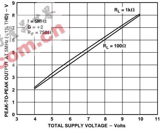
Figure 32. Output Swing vs. Supply
