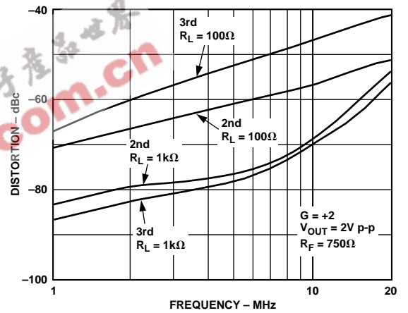
Figure 20. Distortion vs. Frequency; V_S = +5\text{ V}
