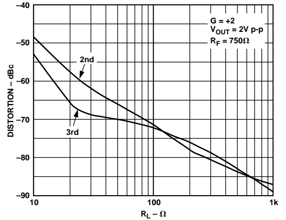
Figure 19. Distortion vs. Load Resistance; V_S = +5\text{ V} , Frequency = 500 kHz
