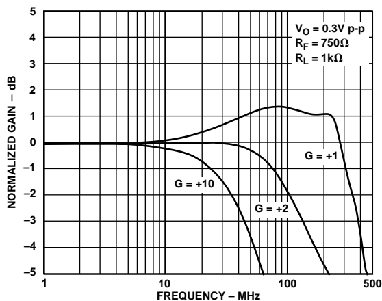
Figure 37. Frequency Response; V_S = +5\text{ V}
