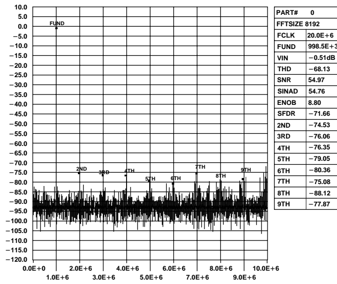
Figure 45. FFT Plot for AD8051 Driving the AD9201 at 1 MHz
