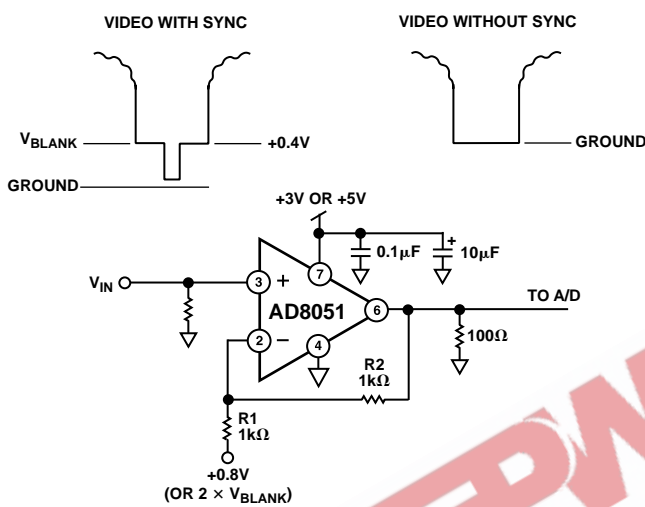
Figure 47. Sync Stripper
