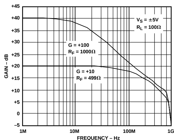
Figure 21. Frequency Response, G = +10 , G = +100
