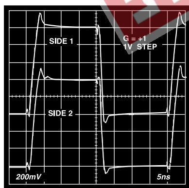
Figure 6. 1 V Step Response, G = +1
