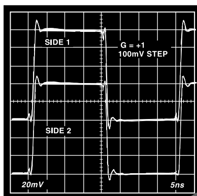
Figure 5. 100 mV Step Response, G = +1
