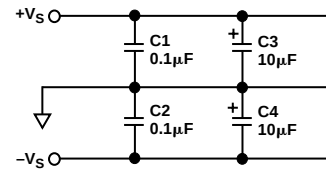
Supply Bypassing
