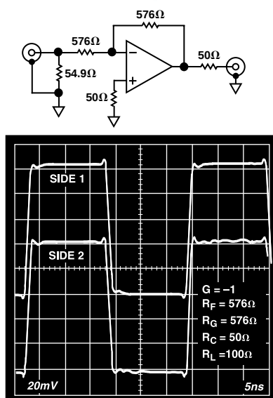
Figure 36. 100 mV Step Response, G = -1
