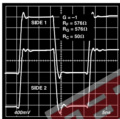
Figure 35. 2 V Step Response, G = -1
