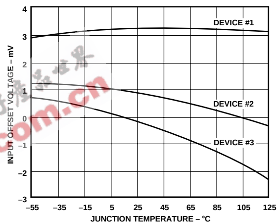
Figure 26. Input Offset Voltage vs. Temperature
