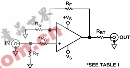
Noninverting Configuration
