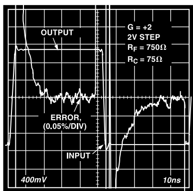
Figure 22. Short-Term Settling Time
