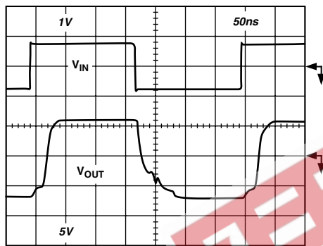
Figure 33. 15% Overload Recovery, Gain = 10 ( R_{FB} = 400 \Omega , R_L = 1 \text{ k}\Omega , V_S = \pm 7.5 \text{ V} )
