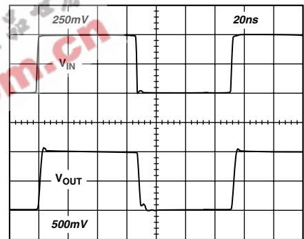
Figure 25. Small Signal Pulse Response, Gain = 2 ( R_{FB} = 750 \Omega , R_L = 150 \Omega , V_S = \pm 7.5 \text{ V} )
