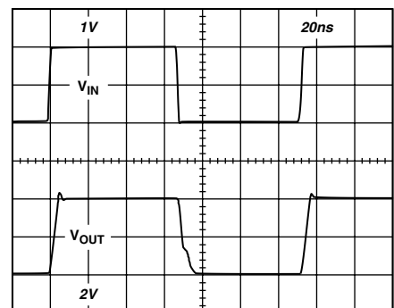
Figure 26. Large Signal Pulse Response, Gain = 2 ( R_{FB} = 750 \Omega , R_L = 150 \Omega , V_S = \pm 7.5 \text{ V} )
