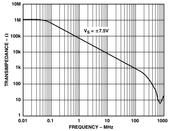
Figure 12. Open-Loop Transimpedance vs. Frequency, R_L = 150 \Omega
