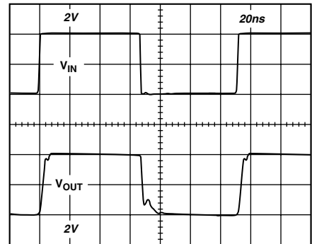
Figure 24. Large Signal Pulse Response, Gain = 1 ( R_{FB} = 5 \text{ k}\Omega , R_L = 150 \Omega , V_S = \pm 7.5 \text{ V} )
