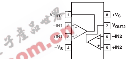
SOIC-8 and SOT-23-8 (RT) AD8034
