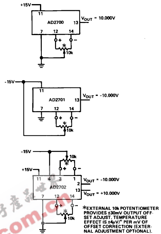
Fine Trim Connections
