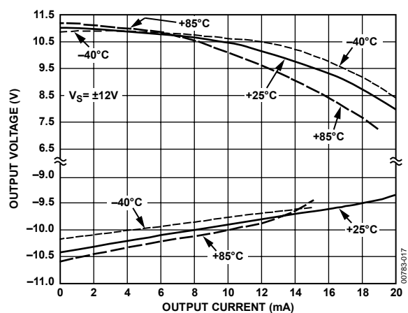
Figure 16. Output Voltage Operating Range vs. Output Current; V_S = \pm 12V
