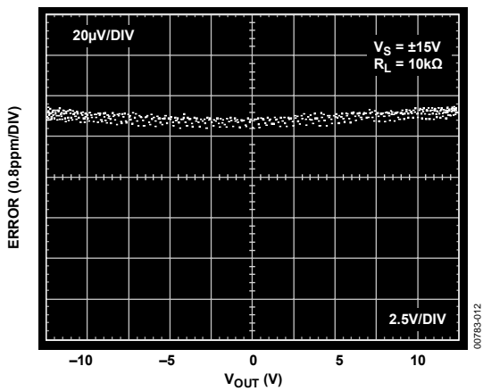
Figure 11. Gain Nonlinearity; V_S = \pm 15V , R_L = 10k\Omega
