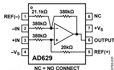
Figure 29. Functional Block Diagram
