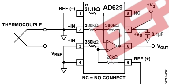
Figure 37. A Gain of 19 Thermocouple Amplifier
