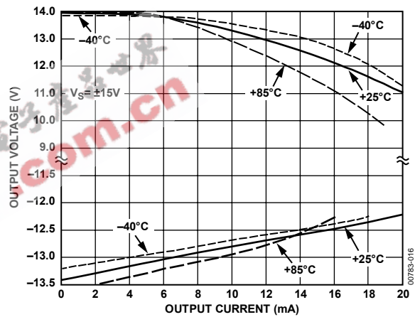
Figure 15. Output Voltage Operating Range vs. Output Current; V_S = \pm 15V
