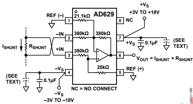
Figure 30. Basic Connections
