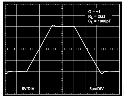
Figure 22. Large Signal Pulse Response
