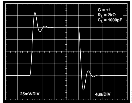
Figure 20. Small Signal Pulse Response
