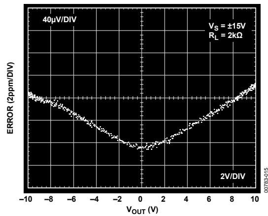
Figure 14. Gain Nonlinearity; V_S = \pm 15V , R_L = 2k\Omega
