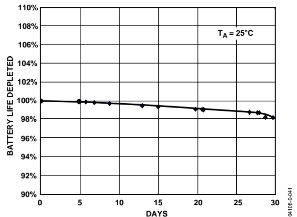
Figure 40. Battery Operating Life Depletion
