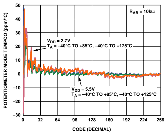
Figure 15. Potentiometer Mode Tempco \Delta V_{ws}/\Delta T vs. Code
