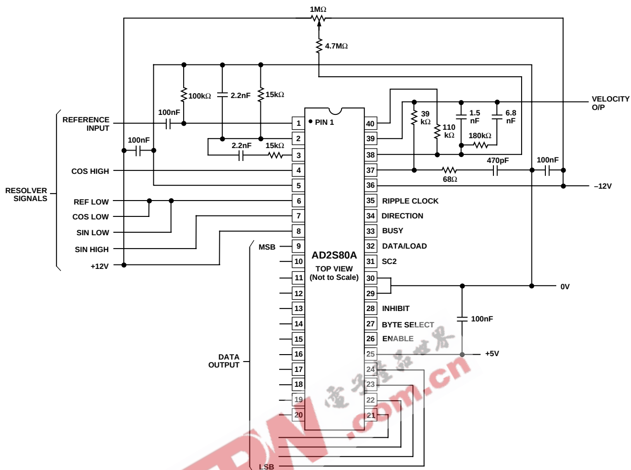
Figure 8. Typical Circuit Configuration
