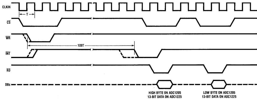
FIGURE 3. Timing Diagram
