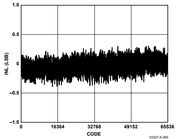
Figure 61. Integral Nonlinearity
