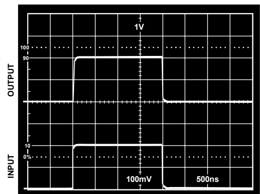
Figure 14. Transient Response, Medium and High Gain
