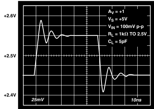
TPC 27. 100 mV Pulse Response, V_S = +5 V
