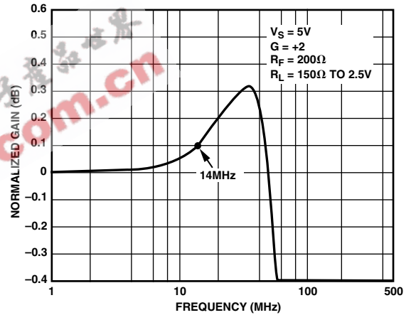
TPC 11. 0.1 dB Gain Flatness
