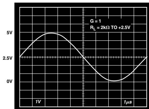
Figure 1. Output Swing: Gain = -1 , V_S = +5 V
