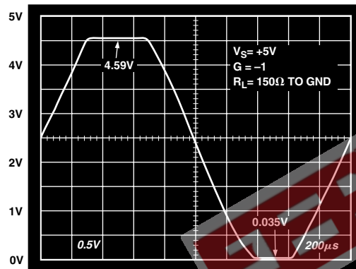
TPC 25b. Output Swing with Load Reference to Negative to Supply
