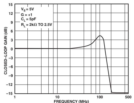
Figure 2. Frequency Response
