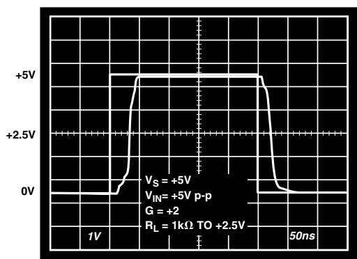
Figure 4. Overdrive Recovery
