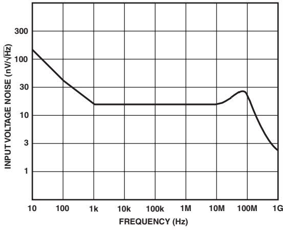
TPC 7. Input Voltage Noise vs. Frequency
