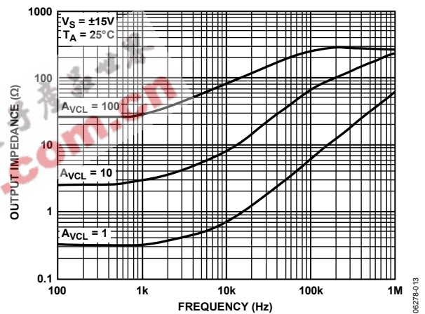
Figure 13. Closed-Loop Output Impedance vs. Frequency
