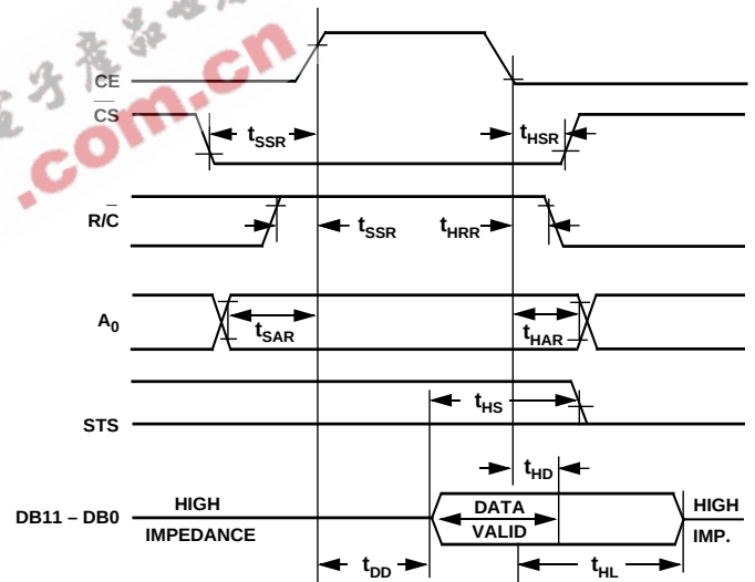
Figure 2. Read Timing
