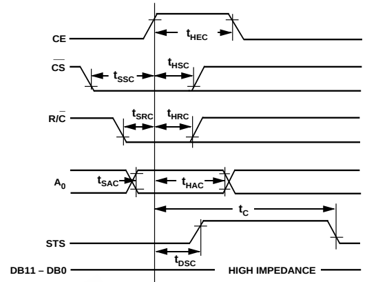
Figure 1. Converter Start Timing
