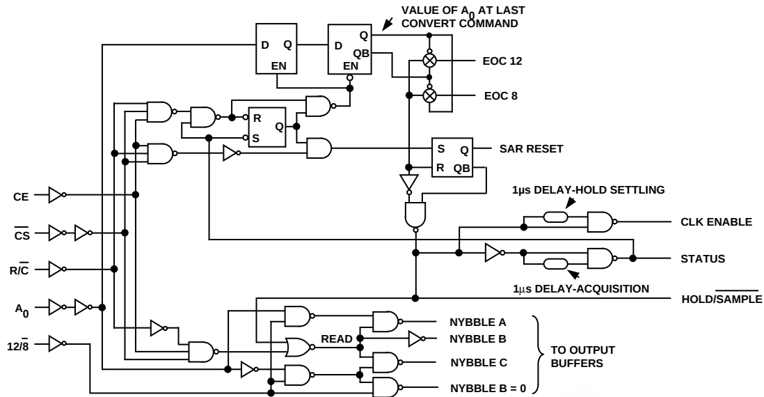
Figure 10. Equivalent Internal Logic Circuitry
