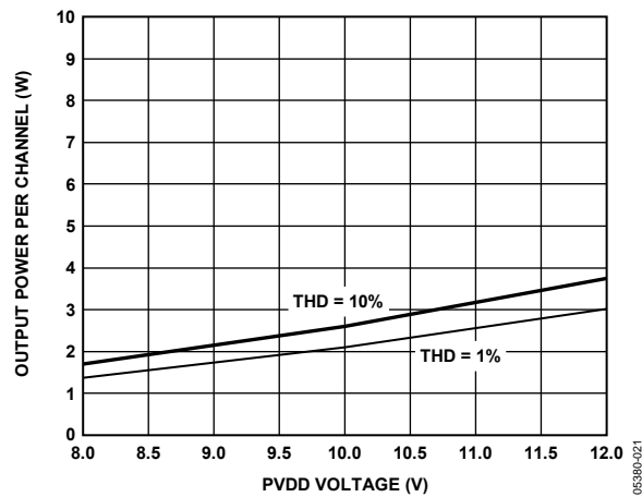
Figure 21. Maximum Output Power vs. PVDD, 8 \Omega Load
