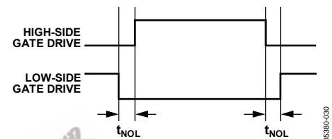
Figure 24. Half-Bridge Nonoverlap Delay Timing
