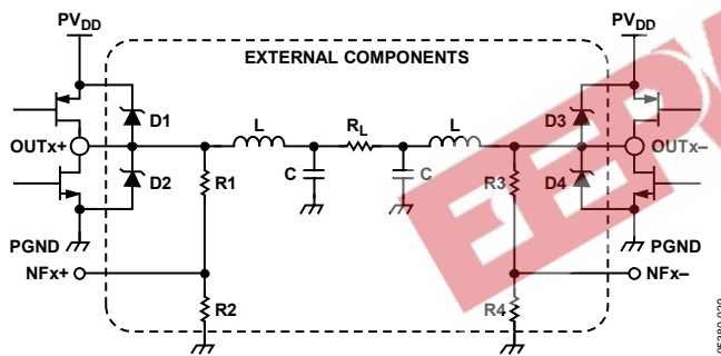
Figure 23. H-Bridge Configuration
