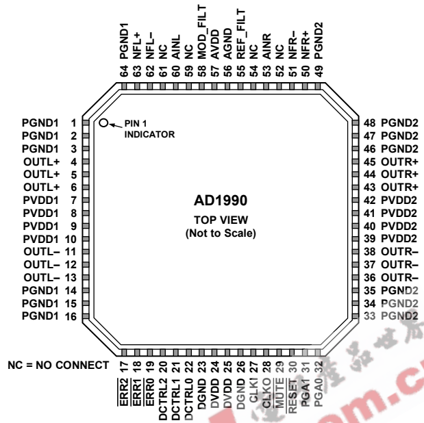
Figure 3. Pin Configuration
