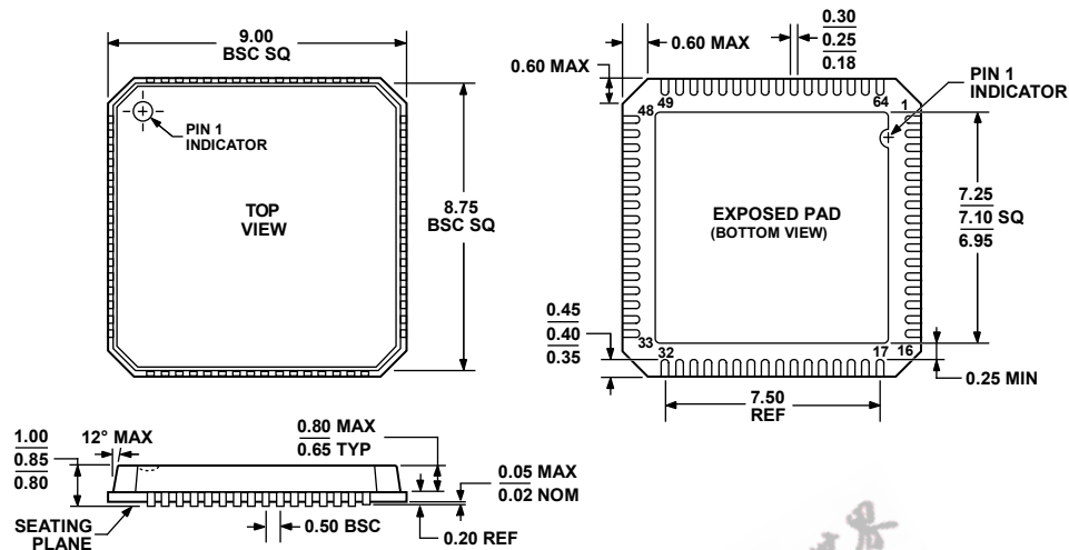
Figure 27. 64-Lead Lead Frame Chip Scale Package [LFCSP_VQ] 9 mm x 9 mm Body, Very Thin Quad (CP-64-3) Dimensions shown in millimeters
