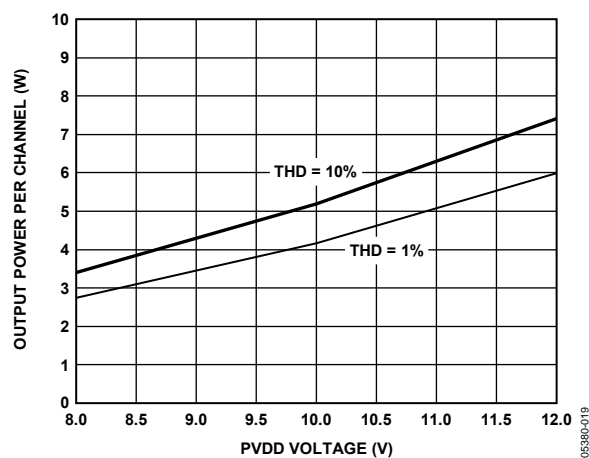
Figure 19. Maximum Output Power vs. PVDD, 4 \Omega Load
