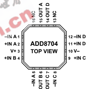
Figure 2. 16-Lead CSP (CP Suffix)
