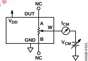
Figure 33. Test Circuit for Common-Mode Leakage Current
