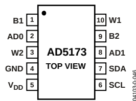
Figure 56. AD5173 Pin Configuration
