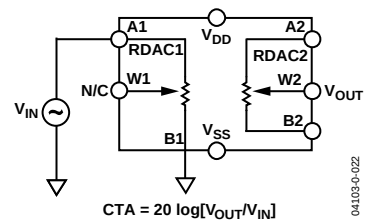
Figure 34. Test Circuit for Analog Crosstalk
