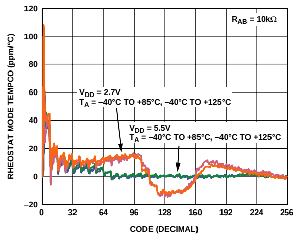
Figure 14. Rheostat Mode Tempco \Delta R_{TWB}/\Delta T vs. Code
