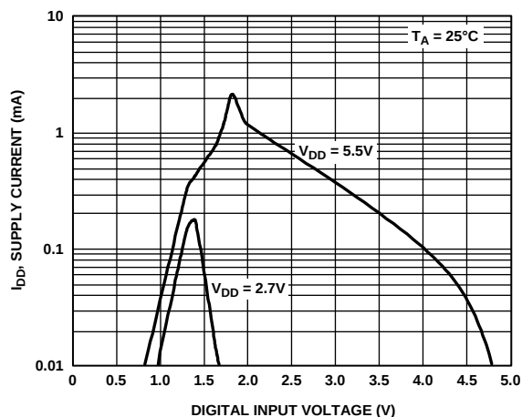
Figure 21. I_{DD} vs. Input Voltage
