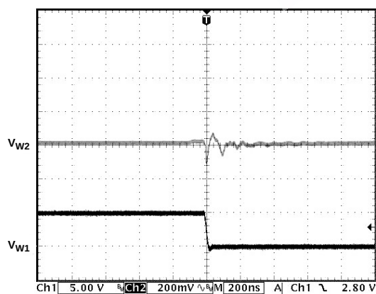
Figure 23. Digital Crosstalk
