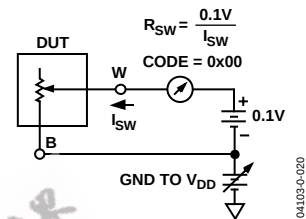
Figure 32. Test Circuit for Incremental On Resistance
