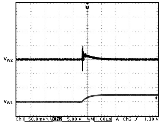
Figure 24. Analog Crosstalk
