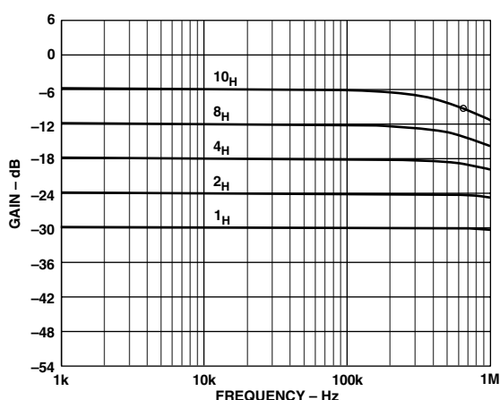
TPC 18. AD5201 10 kΩ Gain vs. Frequency vs. Code
