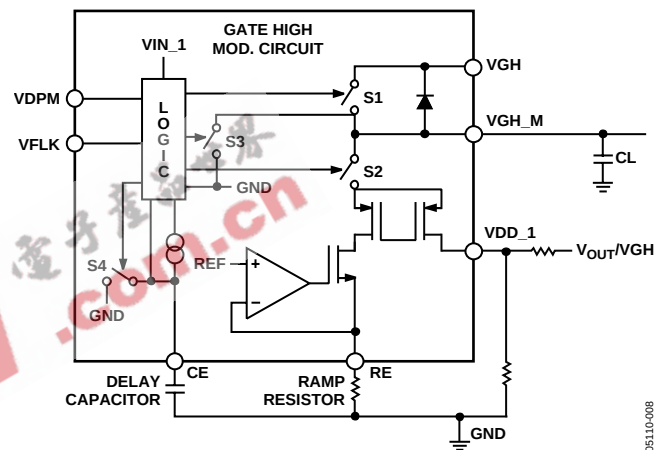
Figure 20. Gate Pulse Modulator Functional Block Diagram
