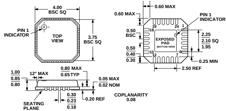
COMPLIANT TO JEDEC STANDARDS MO-220-VGGD-2 Figure 28. 24-Lead Lead Frame Chip Scale Package [LFCSP_VQ] 4 x 4 mm Body, Very Thin Quad (CP-24-1) Dimensions shown in millimeters
