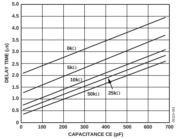
Figure 17. GPM Delay Time vs. CE Capacitance
