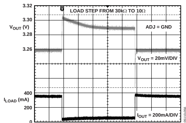
Figure 12. LDO Load Transient Response, V_{OUT} = 3.3\text{ V}
