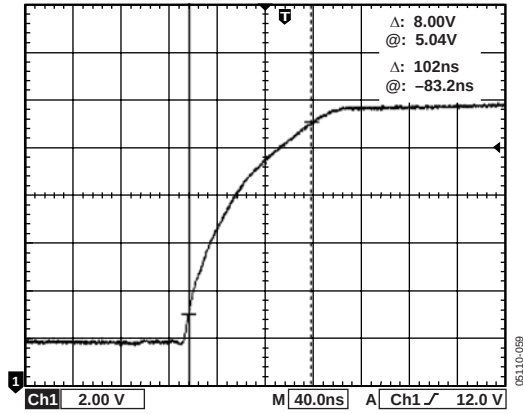
Figure 15. V_{COM} Rising Slew Rate, VDD\_2 = 14 V
