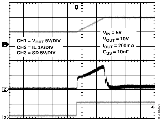
Figure 5. Start-Up Response from Shutdown, C_{SS} = 10\text{ F}
