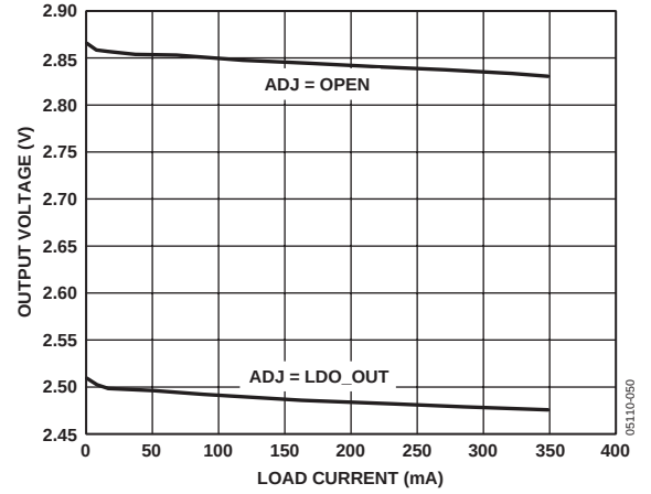
Figure 6. LDO Output Voltage vs. Load Current, V_{IN} = 3.3\text{ V}
