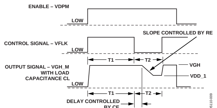
Figure 21. Gate Pulse Modulator Timing Diagram
