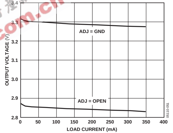
Figure 7. LDO Output Voltage vs. Load Current, V_{IN} = 5\text{ V}
