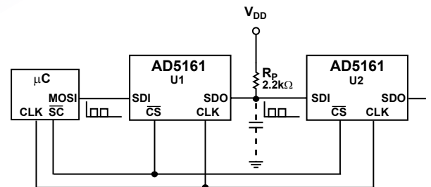
Figure 42. Daisy-Chain Configuration
