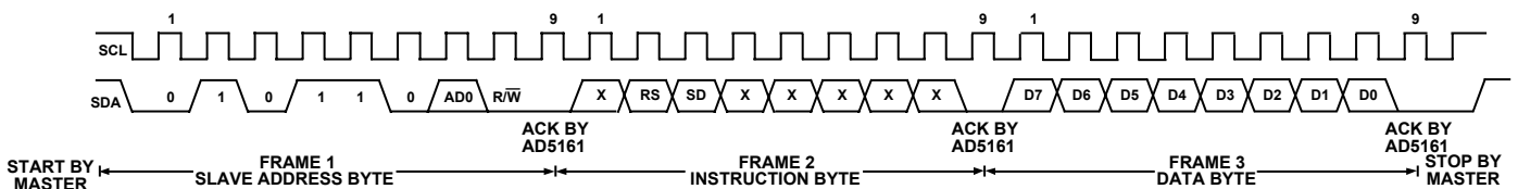
Figure 39. Writing to the RDAC Register
