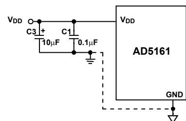
Figure 48. Power Supply Bypassing
