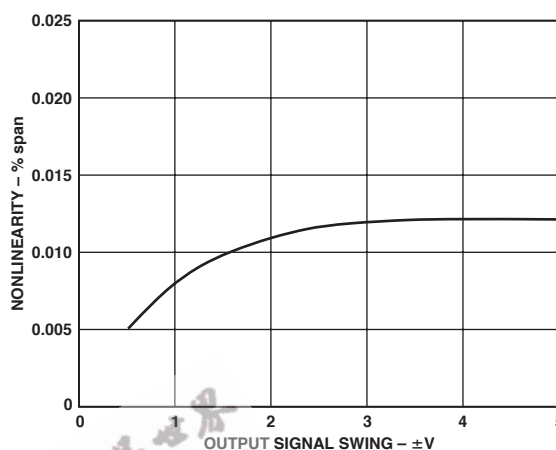
Figure 15. Nonlinearity vs. Signal Swing
