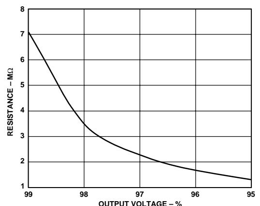
Figure 16. External Resistor Value for Reducing Output Voltage
