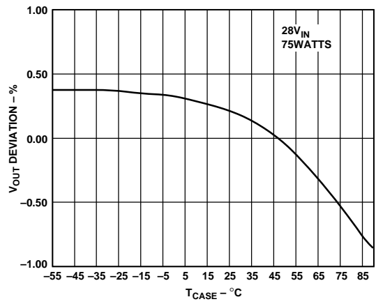
Figure 4. Output Voltage vs. Case Temperature (°C)
