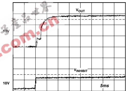
Figure 5. Output Voltage Transient During Turn-On with Minimum Load Displaying Soft Start When Supply Is Enabled
