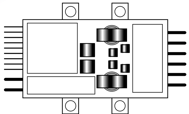
Figure 24. Hot Spots (Shaded Areas) of DC/DC Converter
