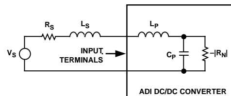
Figure 23. Model of Power Source and POL Converter Connection
