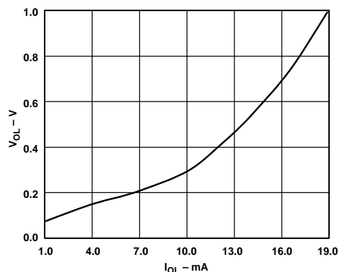
Figure 19. Sink Capability of Status Output
