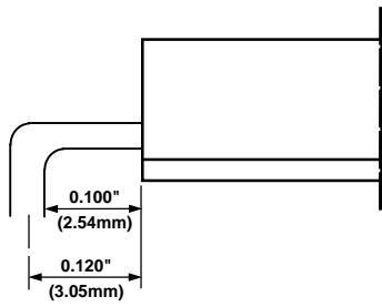
Figure 25. Minimum Bend Radius of 40 Mil (1.02 mm) Pins
