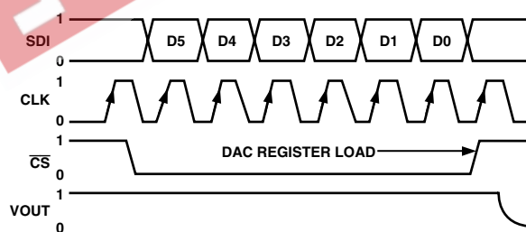
Figure 1b. AD5201 Timing Diagram
