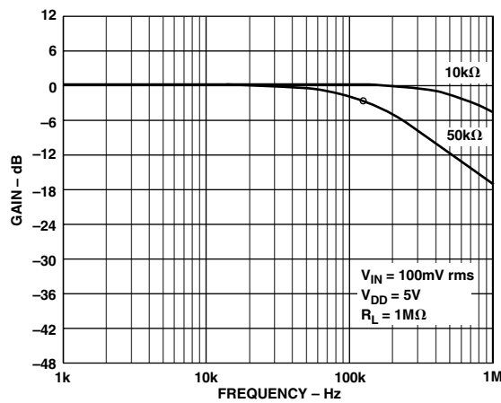
TPC 21. AD5201 -3 dB Bandwidth
