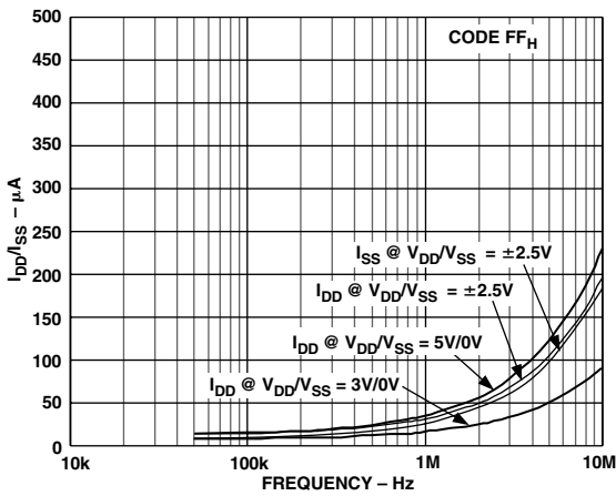
TPC 13. AD5200 10 kΩ Supply Current vs. Clock Frequency
