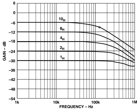
TPC 19. AD5201 50 kΩ Gain vs. Frequency vs. Code
