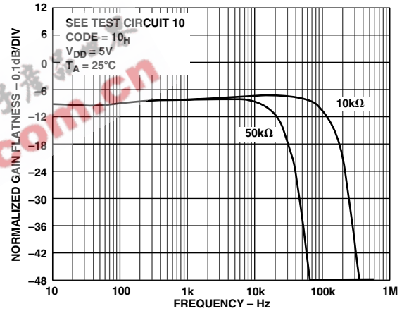
TPC 23. AD5201 Normalized Gain Flatness vs. Frequency
