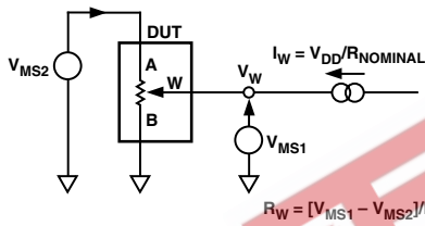
Figure 8. Wiper Resistance Test Circuit
