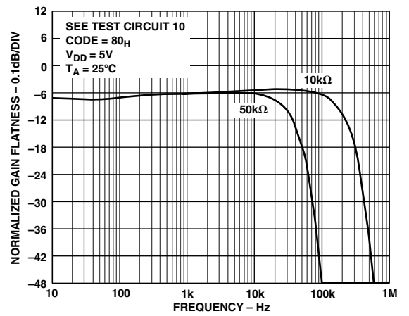
TPC 22. Normalized Gain Flatness vs. Frequency
