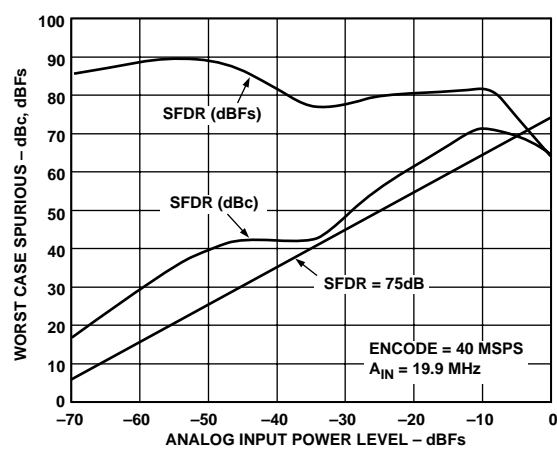
Figure 17. Single Tone SFDR ( A_{IN} @ 19.9) vs. Power Level
