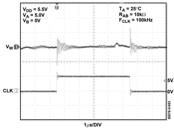
Figure 22. Digital Feedthrough
