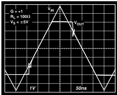
Figure 21. Overload Recovery
