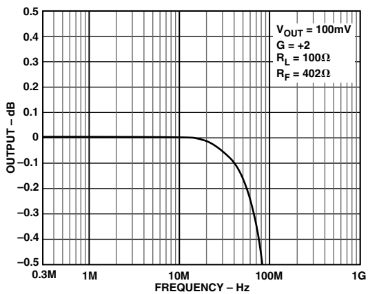
Figure 11. 0.1 dB Flatness
