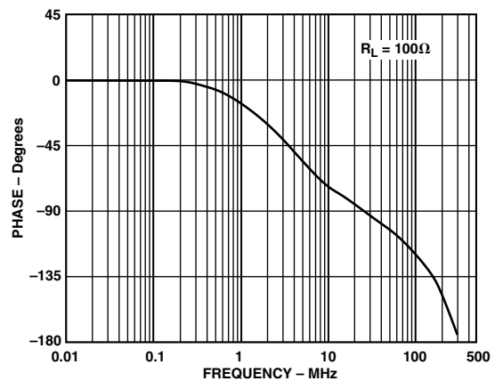
Figure 26. Phase vs. Frequency
