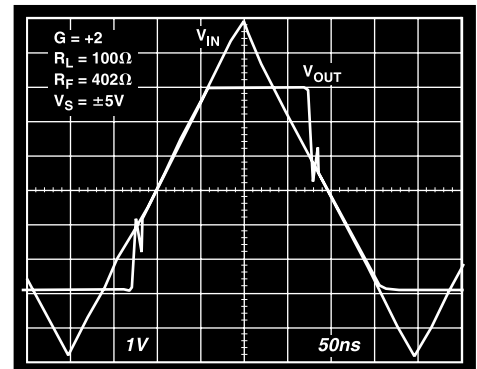
Figure 24. Overload Recovery
