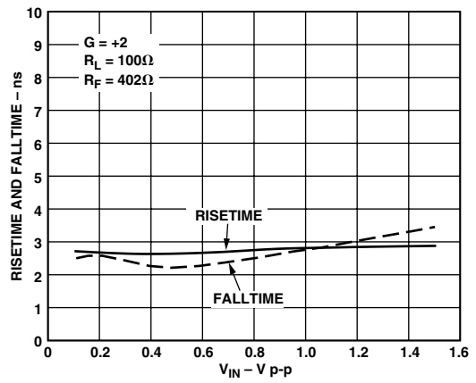
Figure 18. Risetime and Falltime vs. V_{IN}
