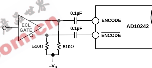
Figure 25. Differential ECL for Encode
