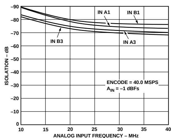
Figure 15. Isolation vs. Frequency
