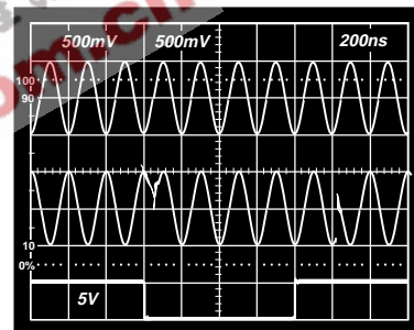
Figure 42. Switching Characteristic for Circuit of Figure 41
