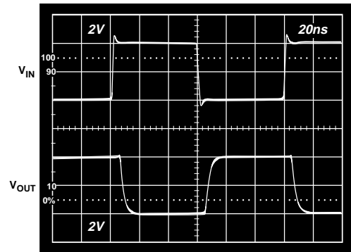
Figure 24. Large Signal Pulse Response, Gain = -1, ( R_F = 698 \Omega , R_L = 150 \Omega , V_S = \pm 5 \text{ V} )
