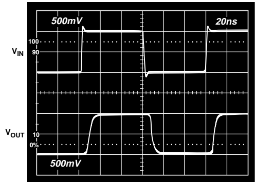
Figure 20. Small Signal Pulse Response, Gain = +1, ( R_F = 2\text{ k}\Omega , R_L = 150\Omega , V_S = \pm 5\text{ V} )
