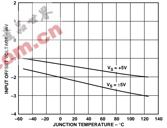
Figure 7. Input Offset Voltage vs. Junction Temperature
